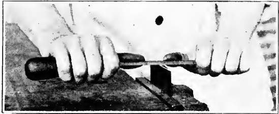
FIG. 117. DRAWFILING A SCRAPER.
